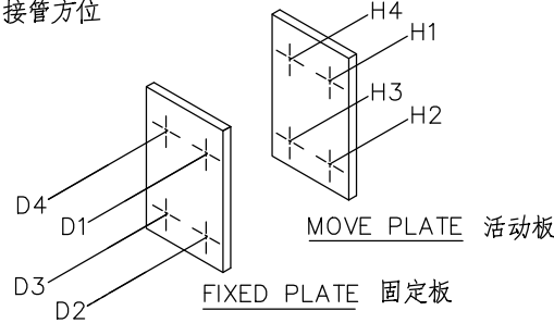
CONNECTION LOCATIONS
